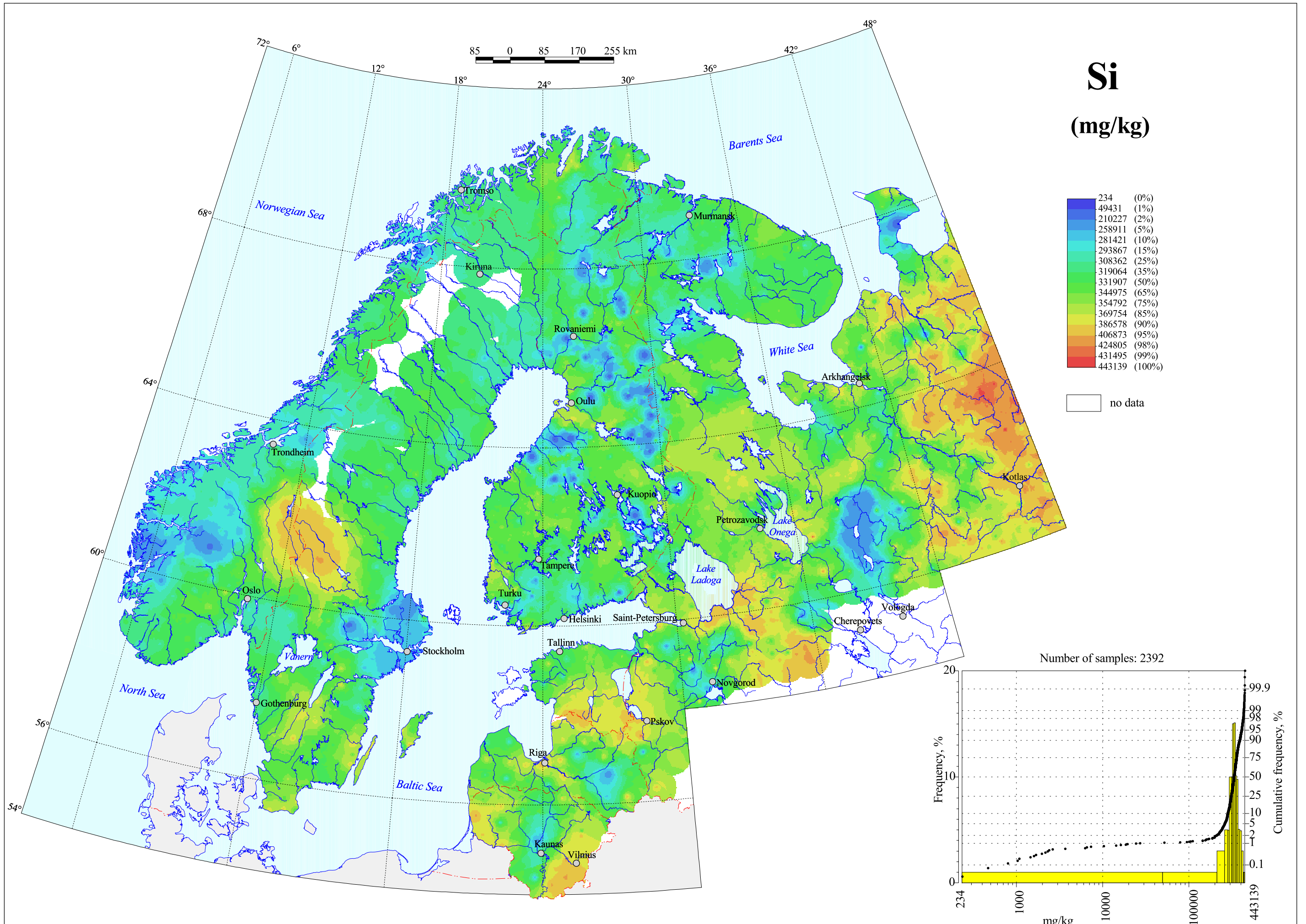
Silicon in C-horizon, Grain Size <2 mm, Total Content
